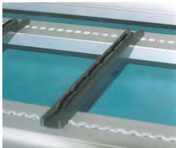
Anti-vibration plastic card guide in aluminum extrusion cage with blue anodize finish.
