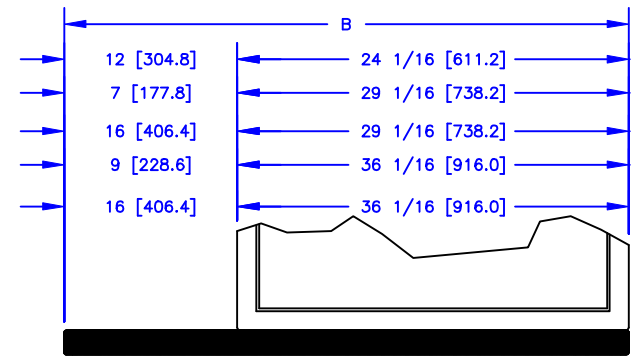
EXTENDED CABINET TRUCK TRIPLE WIDTH
