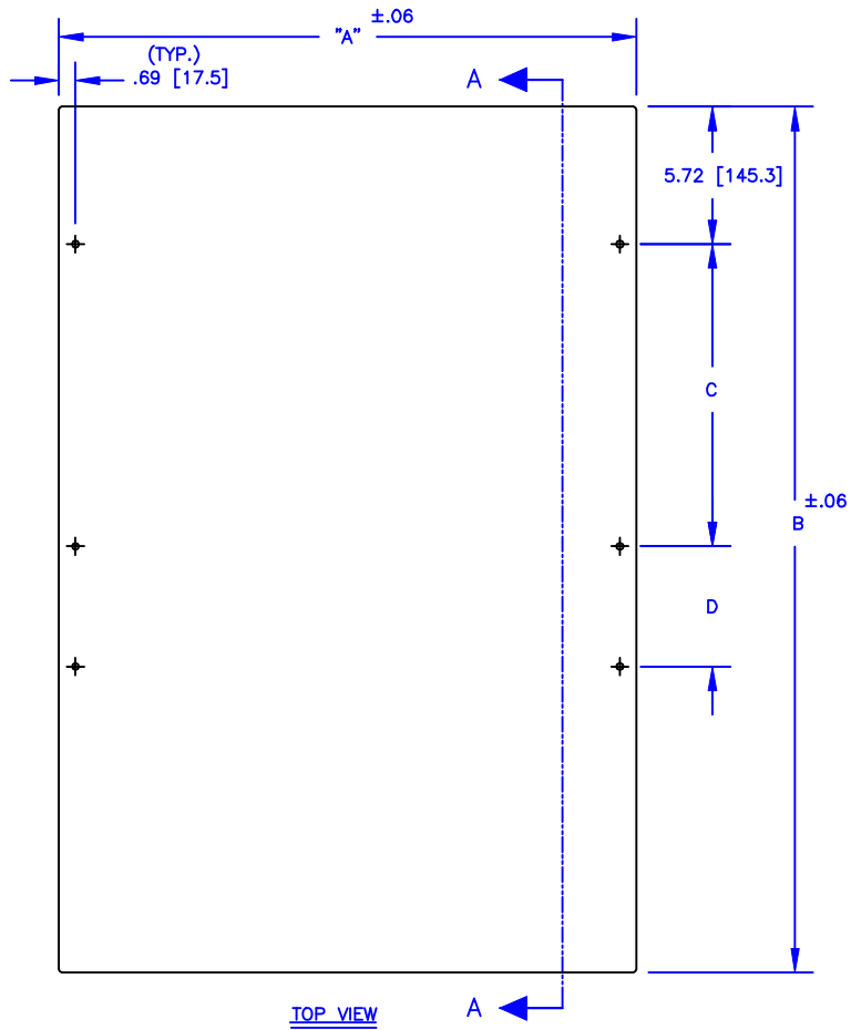
EXTENDED CABINET TRUCK SINGLE WIDTH
