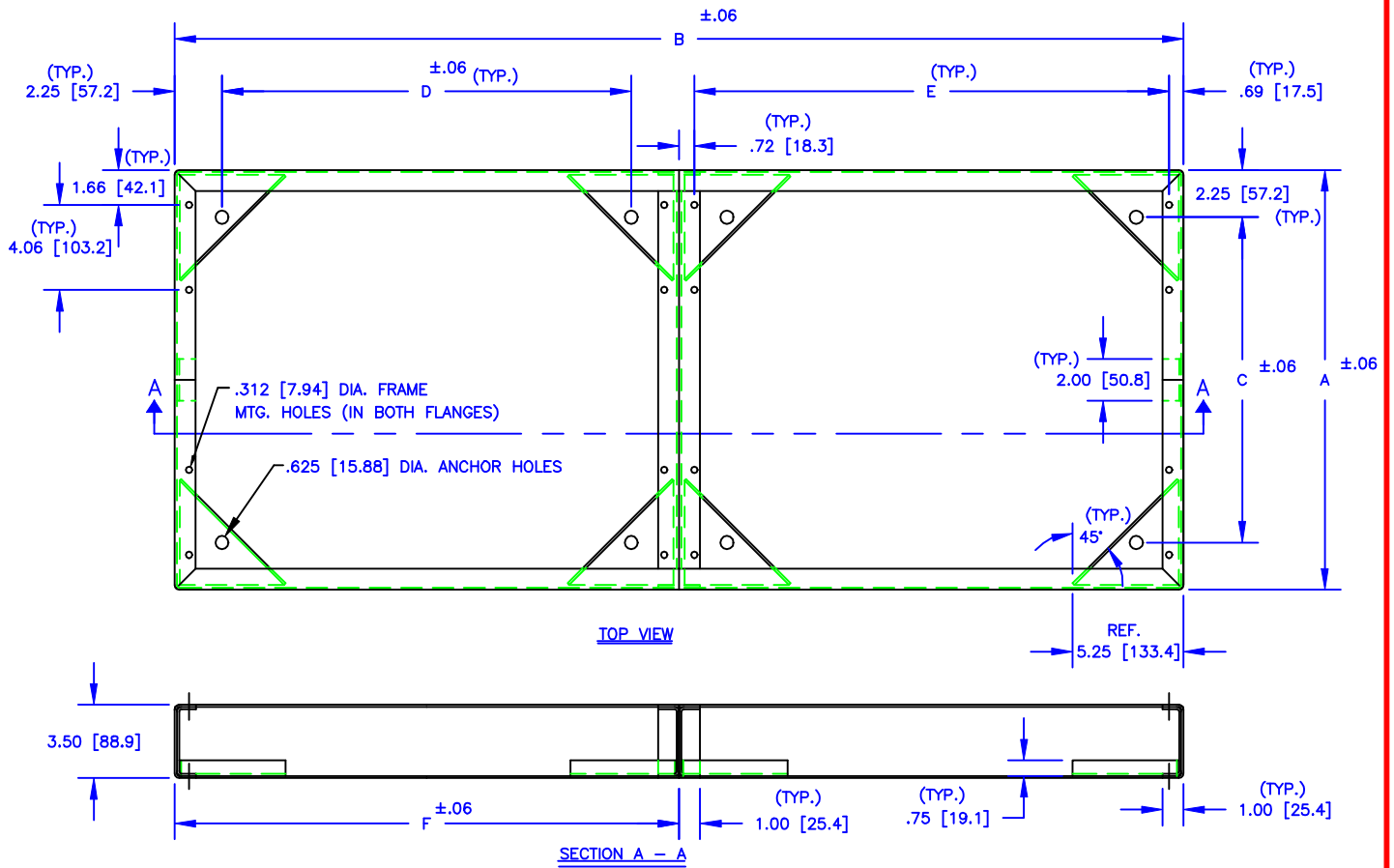
FLUSH FRAME BASES
