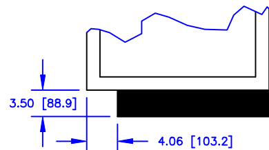
RECESSED BASE
