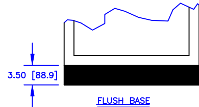
FLUSH BASE
