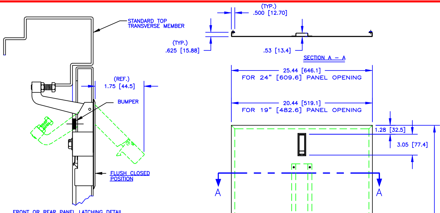
FRONT OR REAR PANEL LATCHING DETAIL
