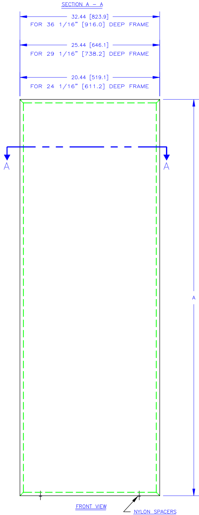
NYLON SPACERS
