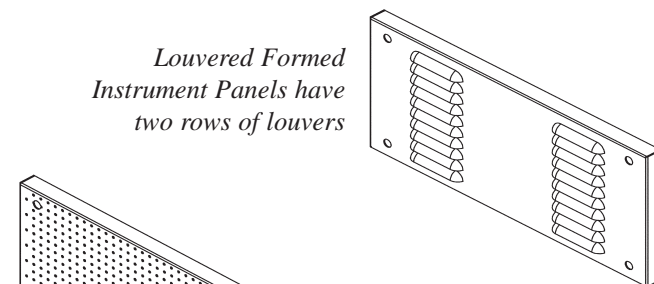
Perforated panels are ideal for releasing heat and complying with codes restricting size of openings
