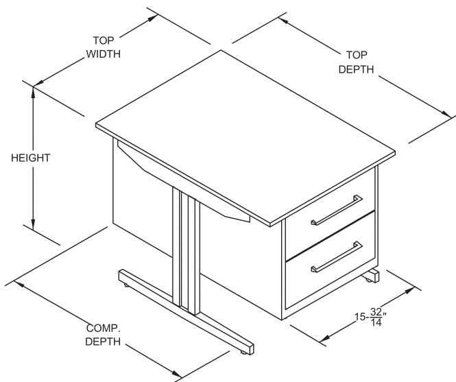
Pedestal Desk Work Station with size dimensions
