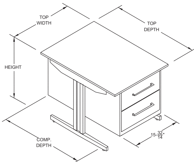
Pedestal Desk Work Station with size dimensions
