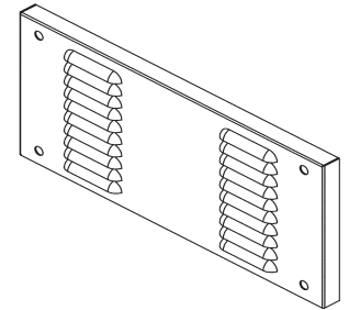
Louvered Formed Instrument Panels have two rows of louvers
