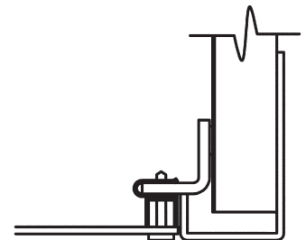
Panel Shim in place between flat panel and panel mounting angle
